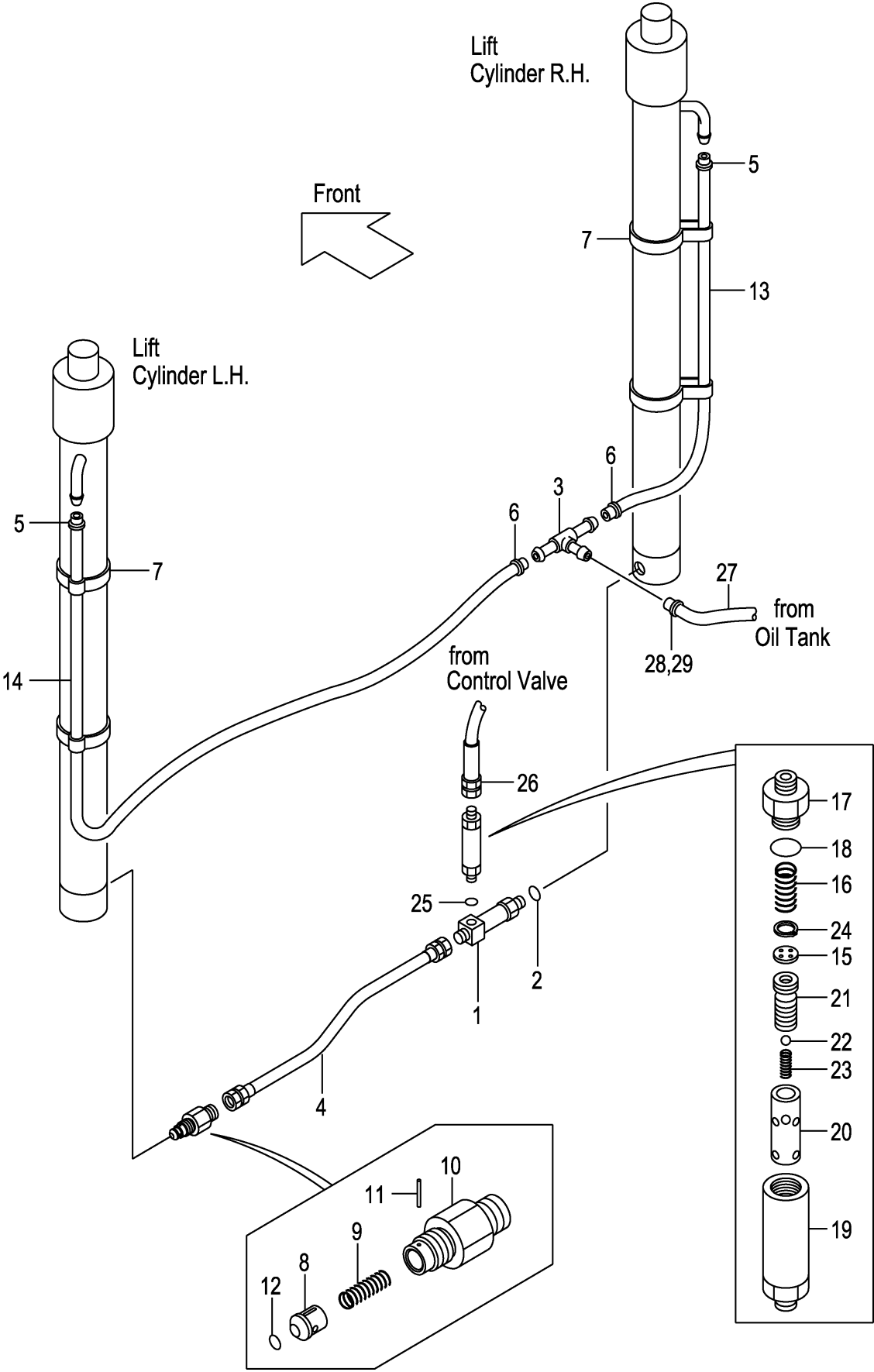
FIG.226 MAST PIPING [VMCN9] (M7G28440)
