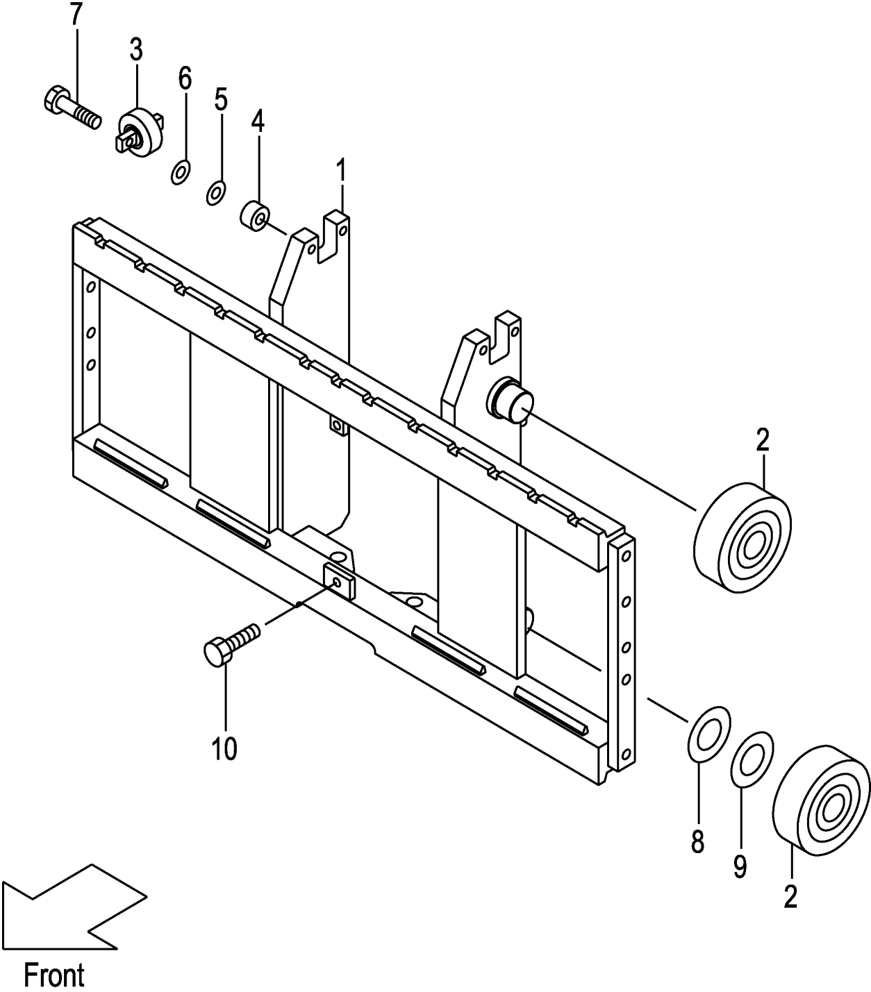
FIG.215 LIFT BRACKET [VFHMCN5] (M7G20910)
