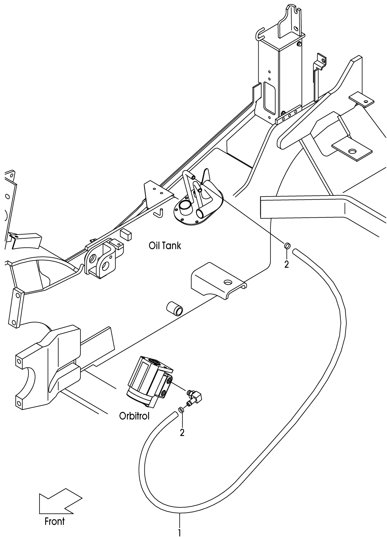
FIG.116 HYDRAULIC LINE (MAIN)(3/4) (F7G27660)
