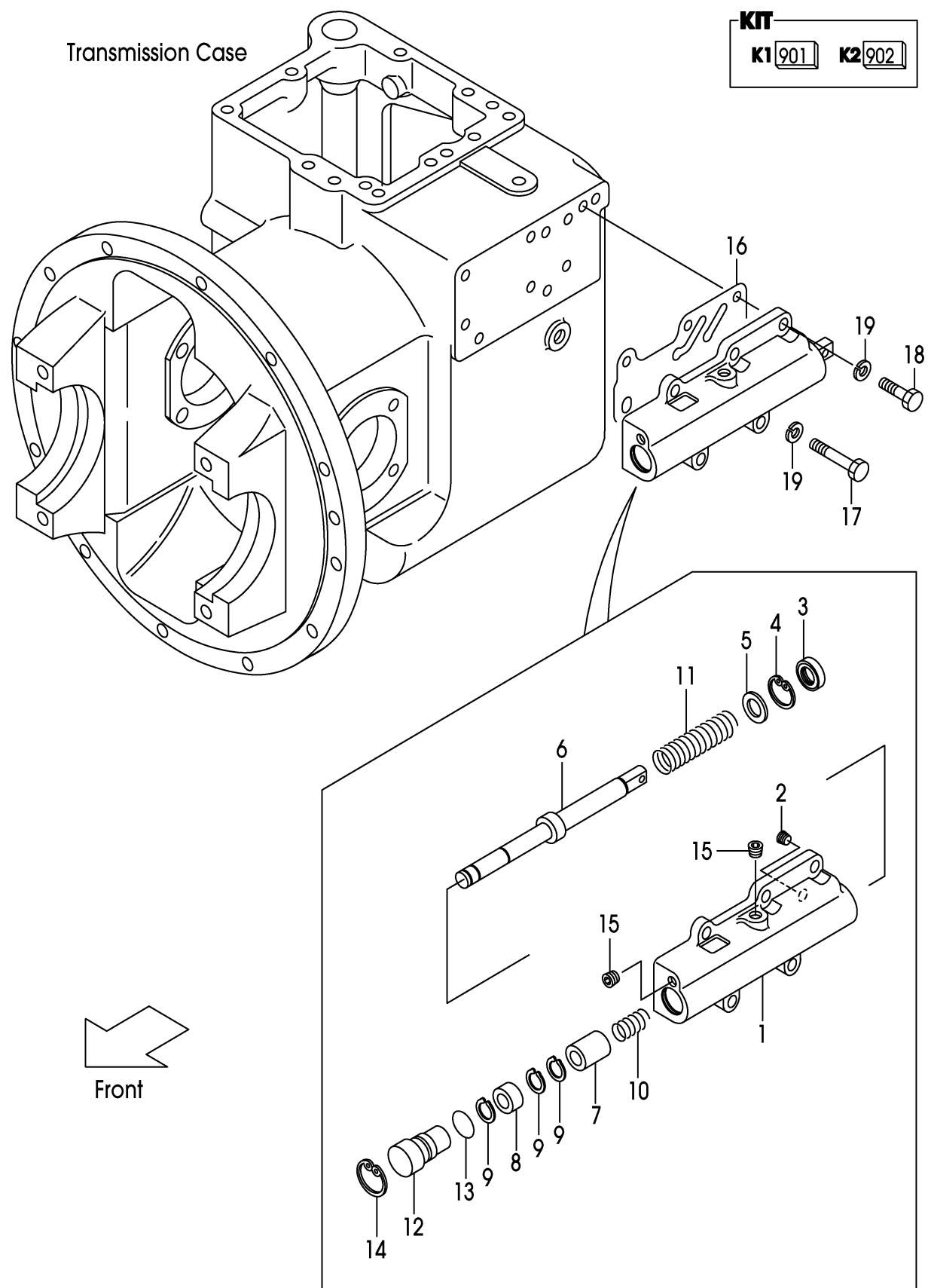
FIG.47 INCHING VALVE (F7G22570)
