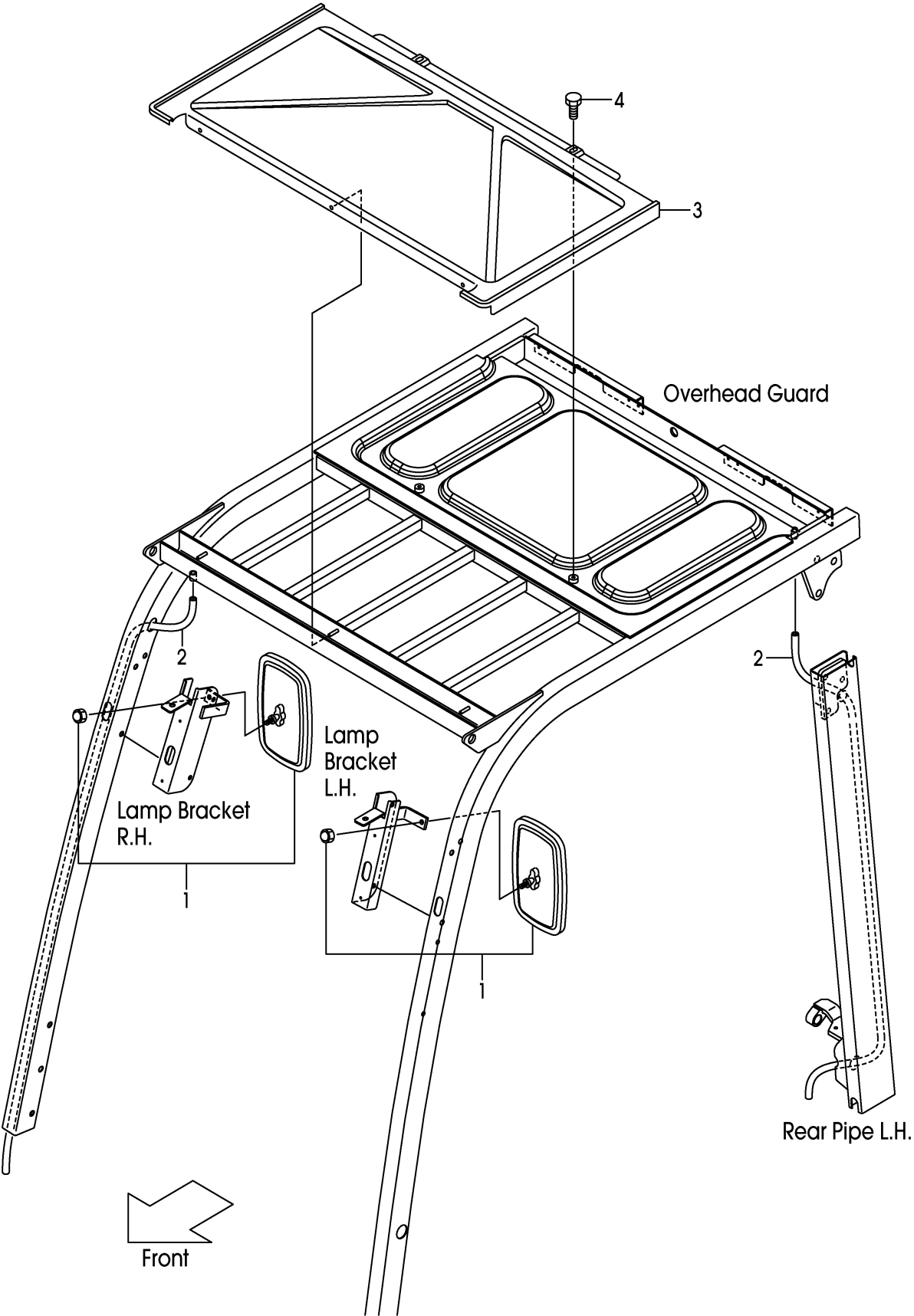
FIG.73 HEAD GUARD PARTS (F7G251A0)
