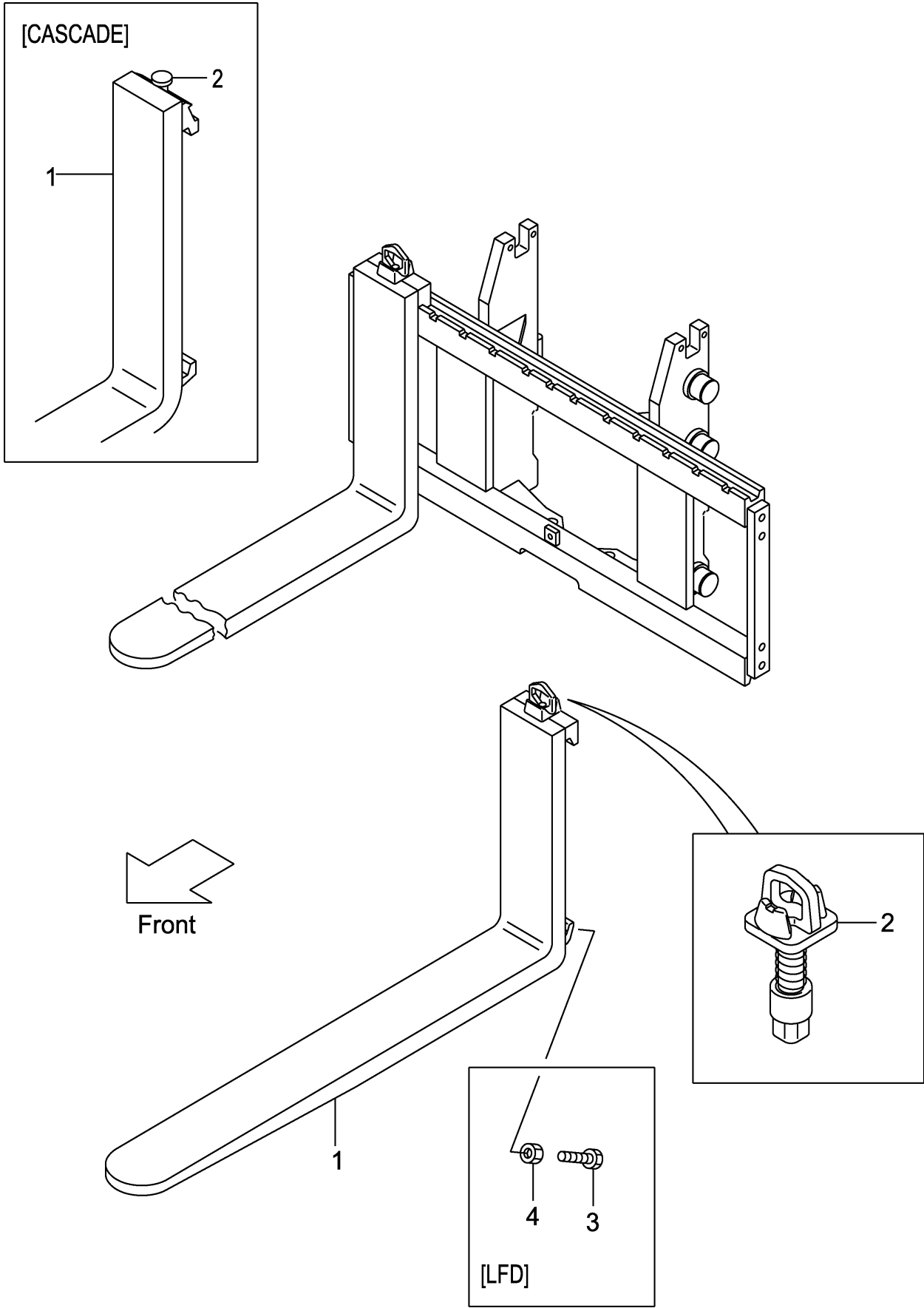
FIG.227 FORK [VFMCN9] (M7G28150)
