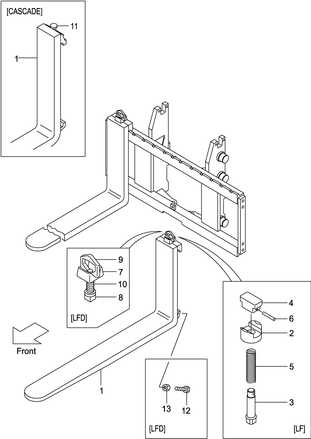
FIG.207 FORK [VFMCN5] (M7G28140)
