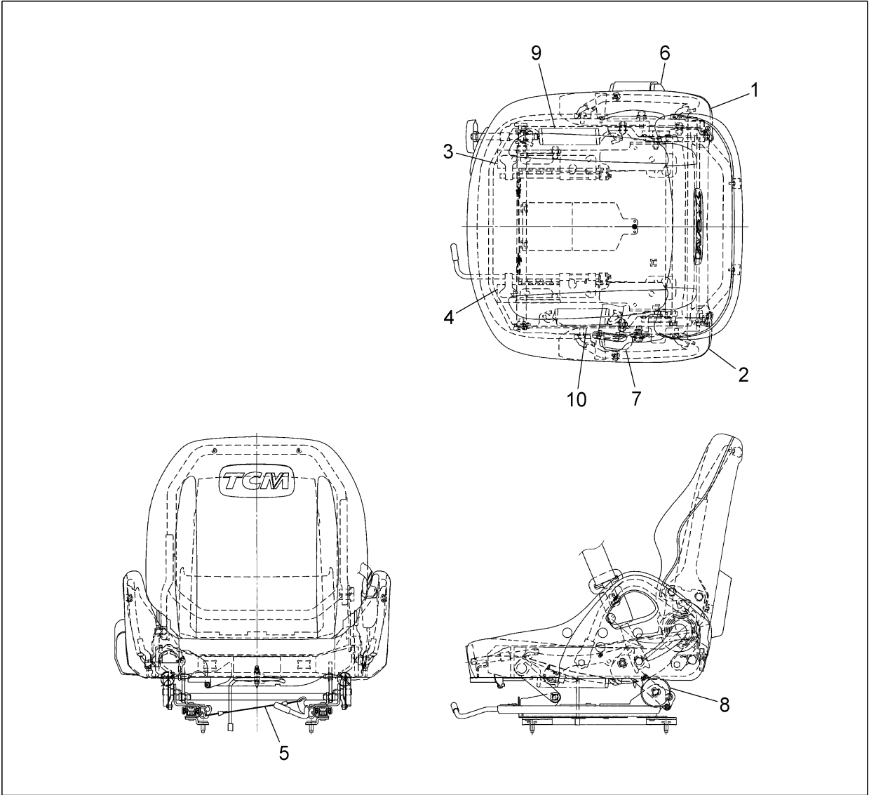
FIG.100 SEAT (F7G26810)
