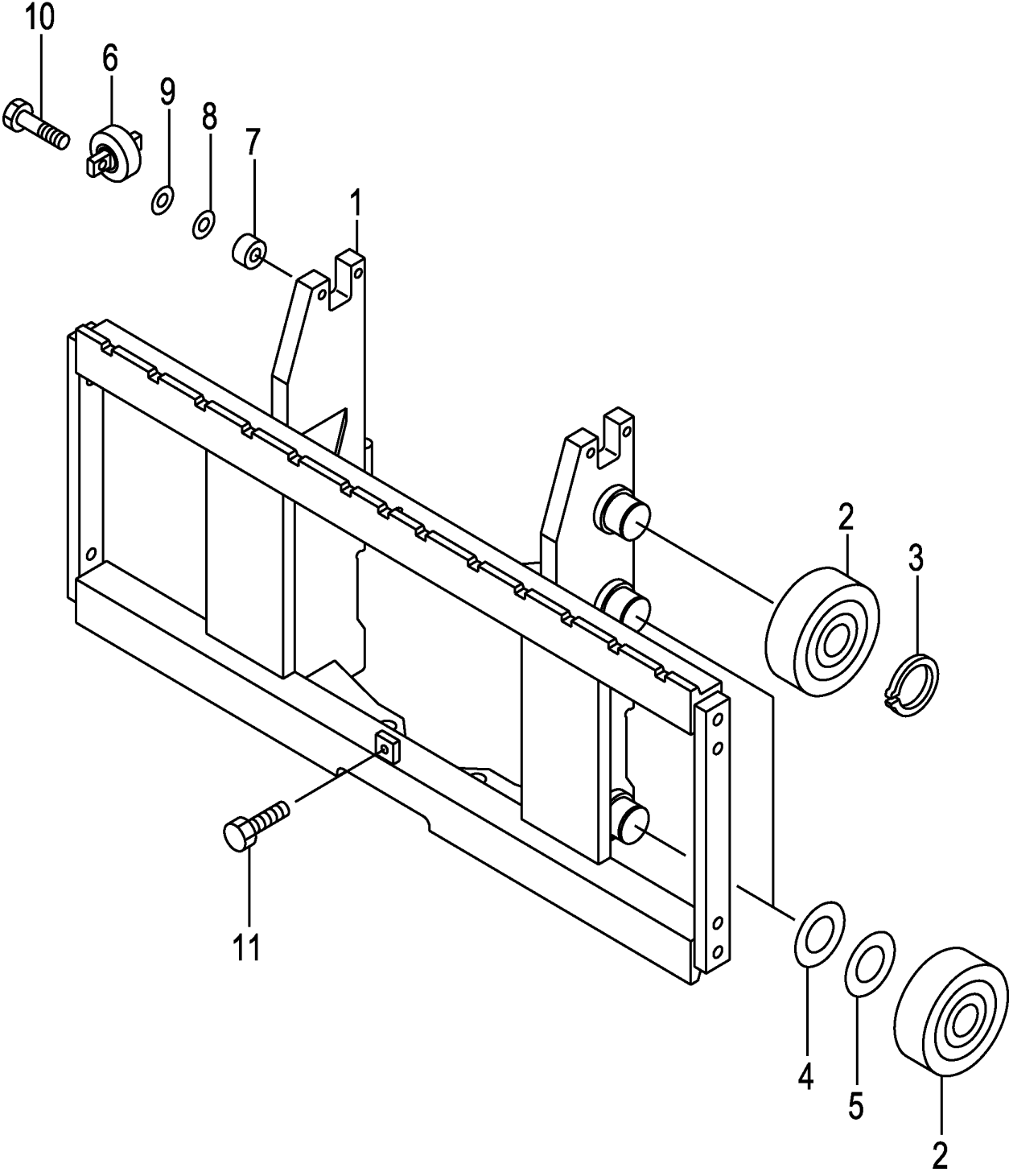
FIG.208 LIFT BRACKET [VFMCN5] (M7G20610)
