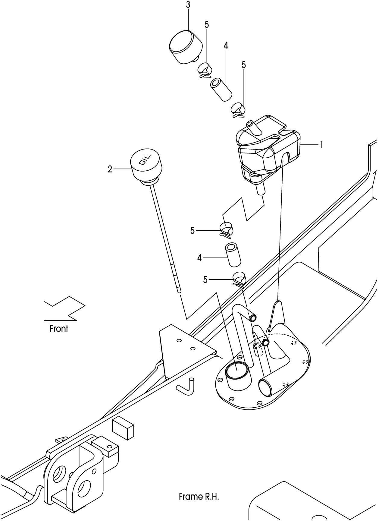
FIG.87 OIL CAP & LEVEL (F7G26130)
