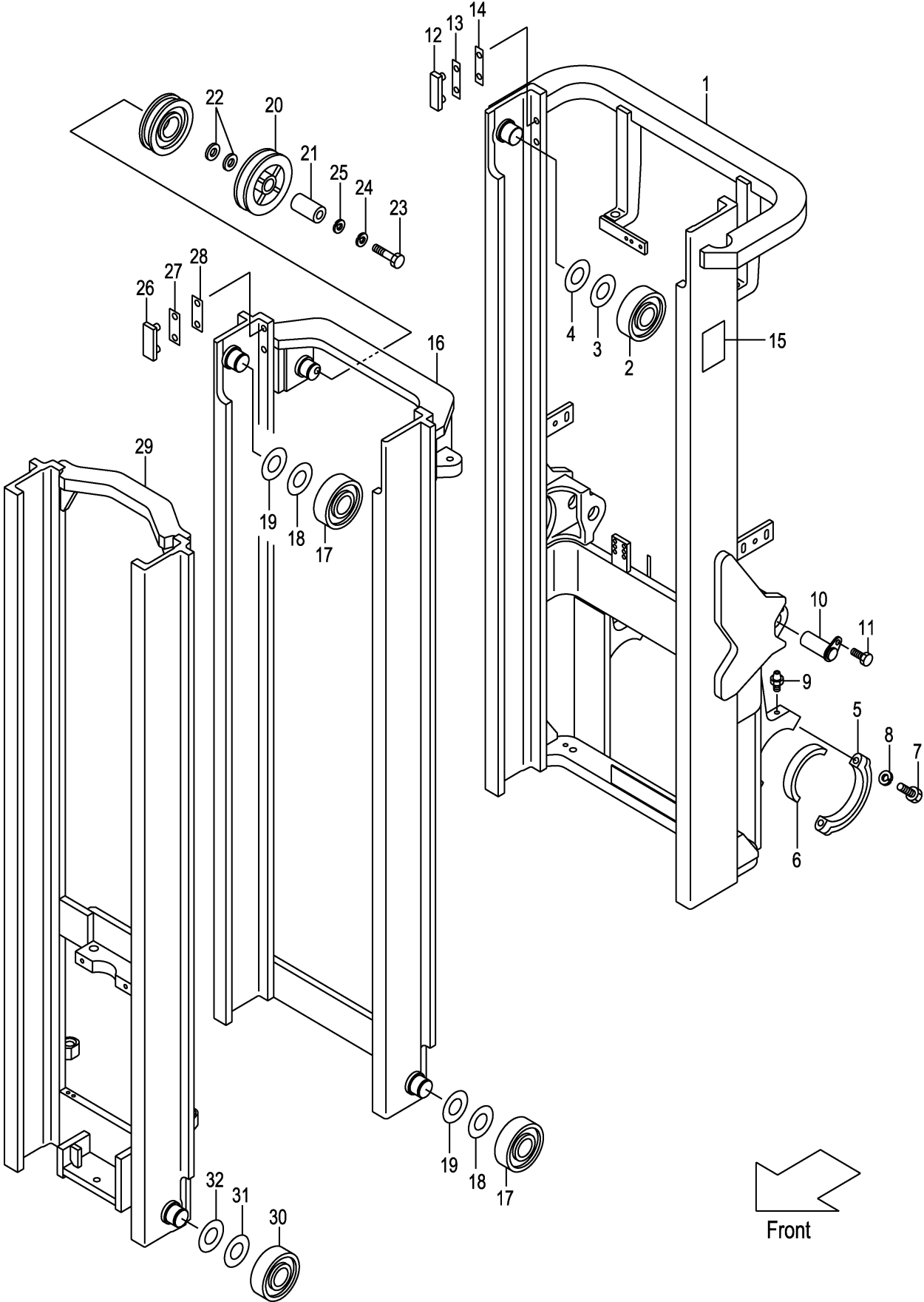
FIG.237 MAST [VFHMCN9] (M7G20740)
