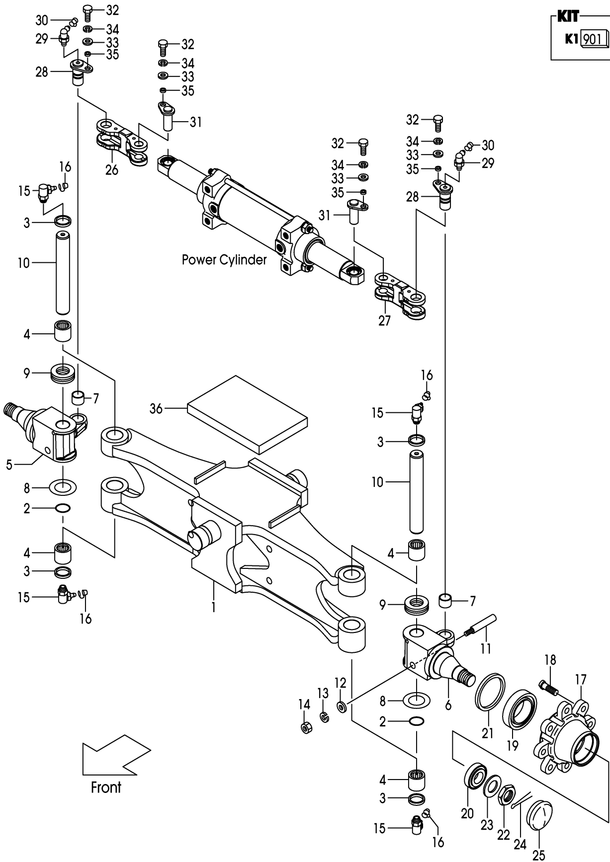
FIG.58 STEERING AXLE (F7G24320)
