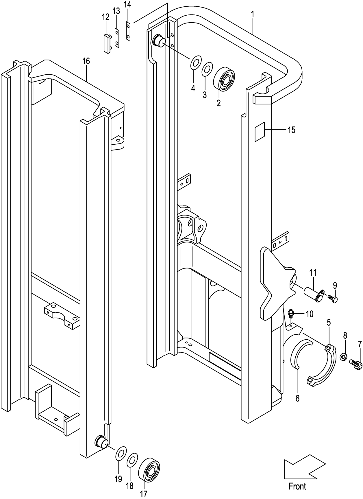
FIG.210 MAST [VFMCN5] (M7G20410)
