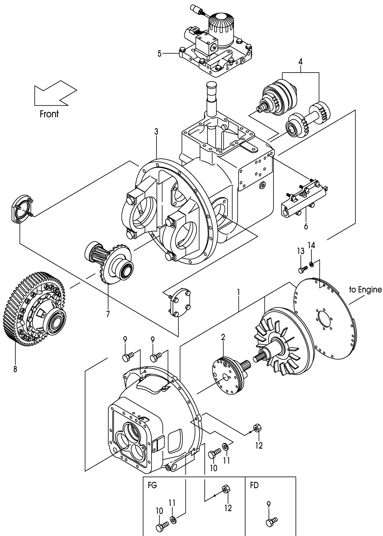
FIG.41 DRIVE UNIT MOUNT (F7G22510)
