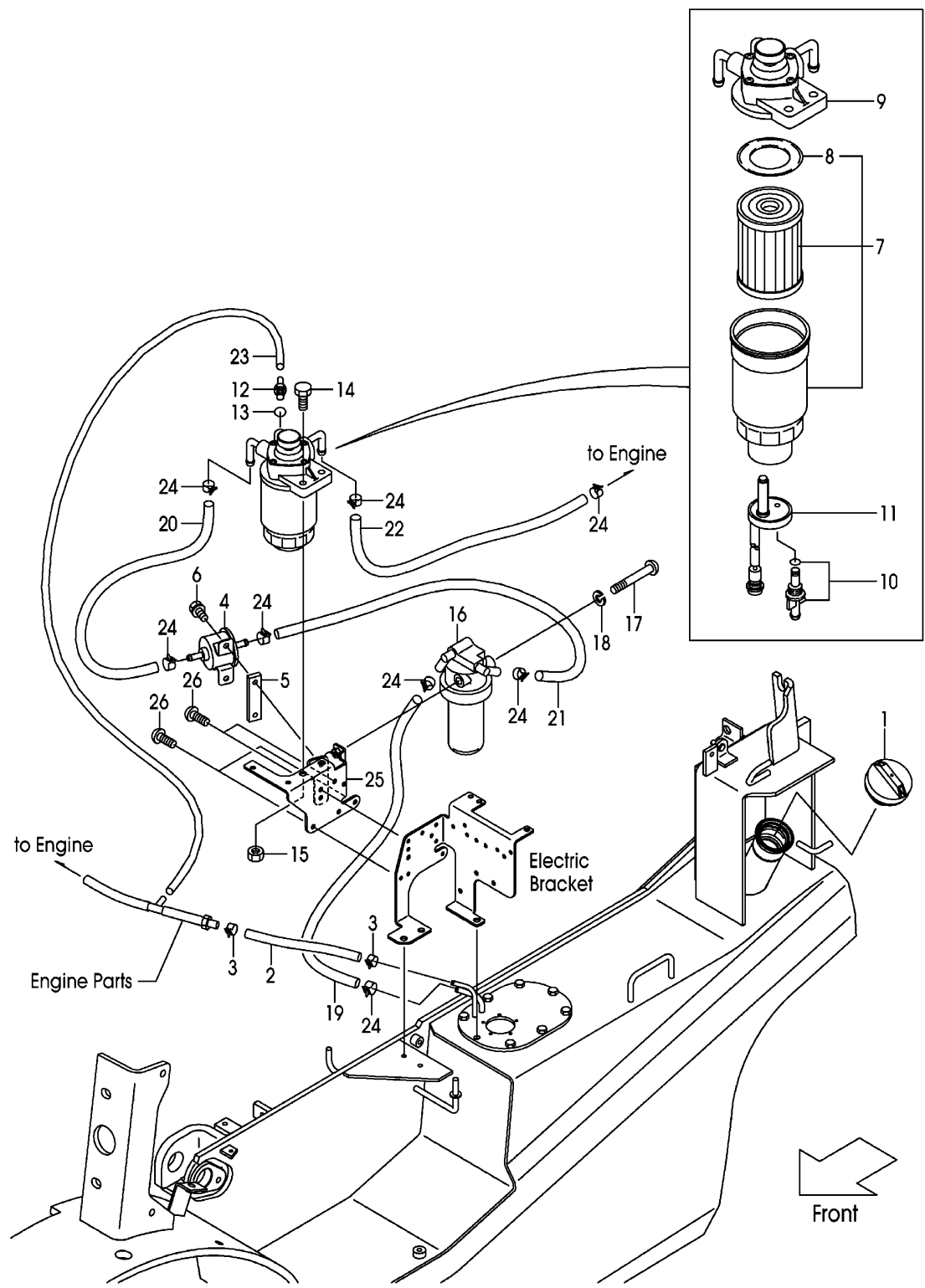
FIG.21 FUEL SYSTEM (F7J32220C)
