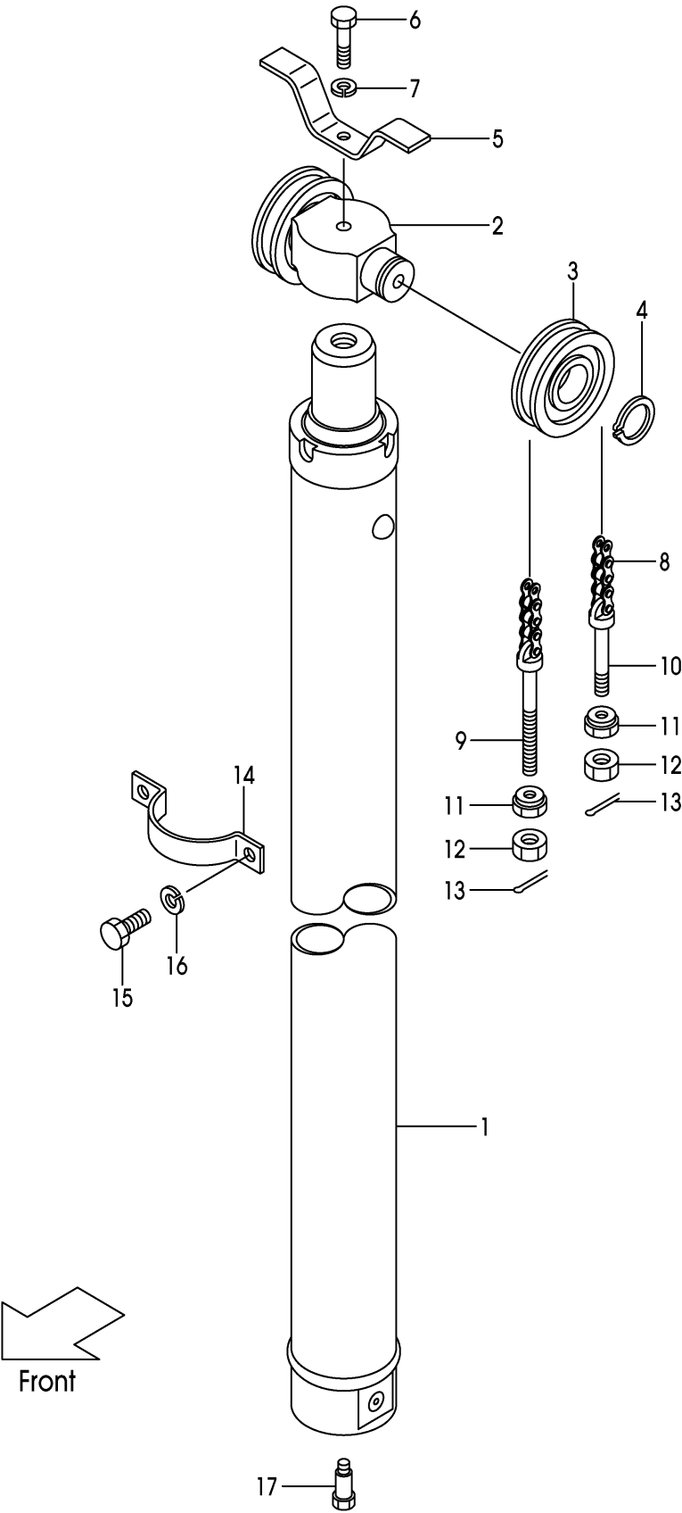
FIG.218 LIFT CYLINDER (FRONT) [VFHMCN5] (M7G20810)
