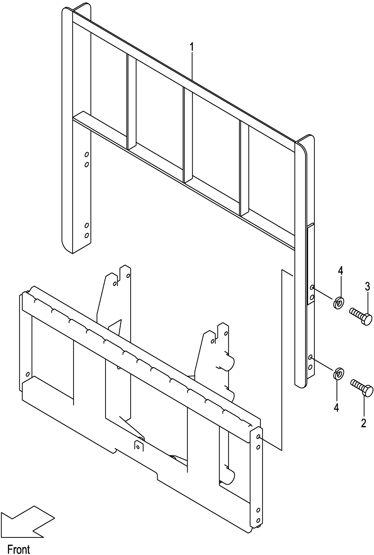
FIG.223 BACKREST [VMCN9] (M7G28240)
