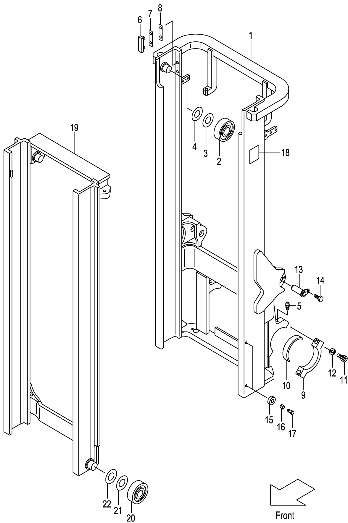
FIG.224 MAST [VMCN9] (M7G28320)
