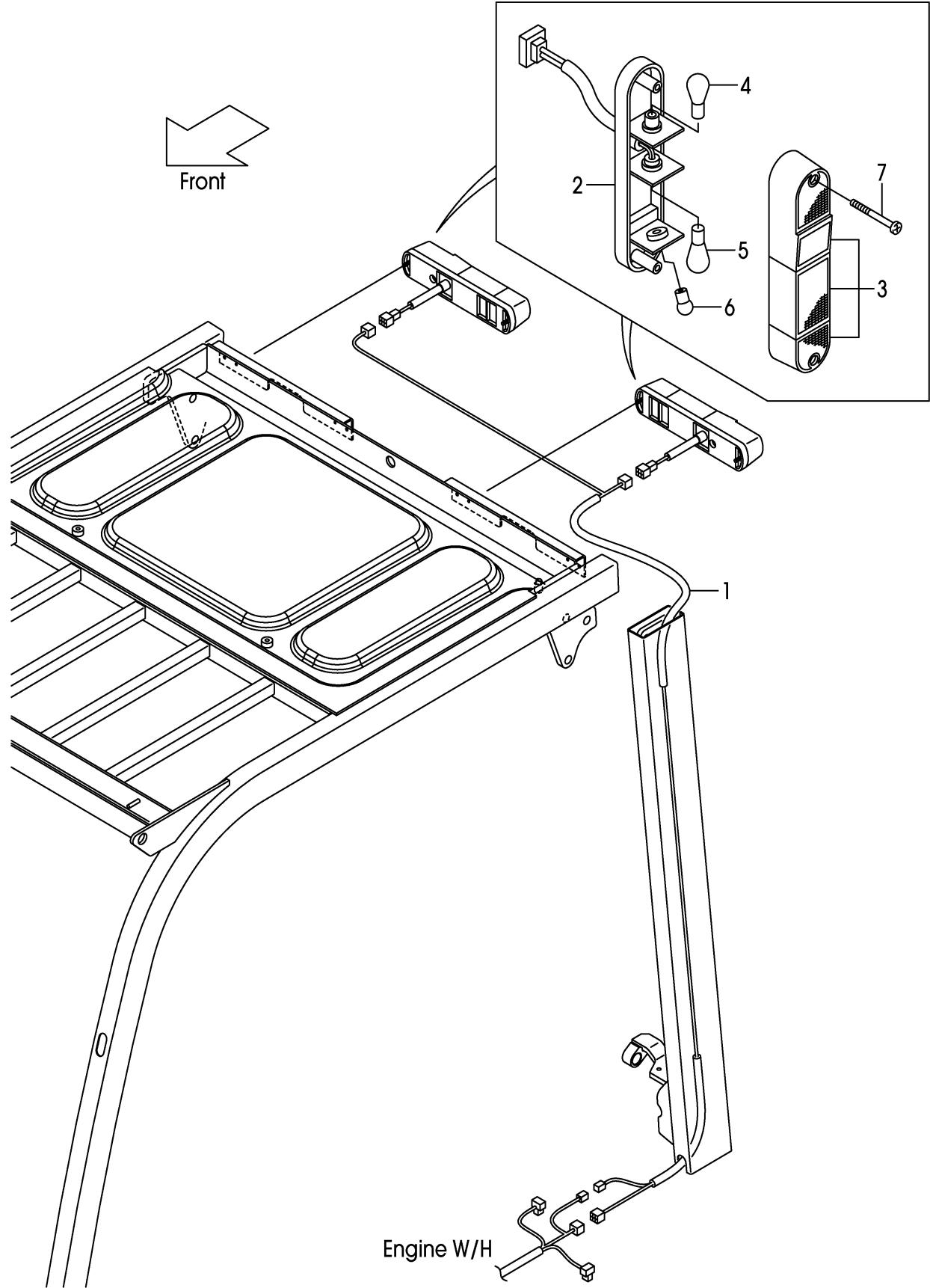
FIG.39 REAR COMBINATION LAMP (F7G224C0)
