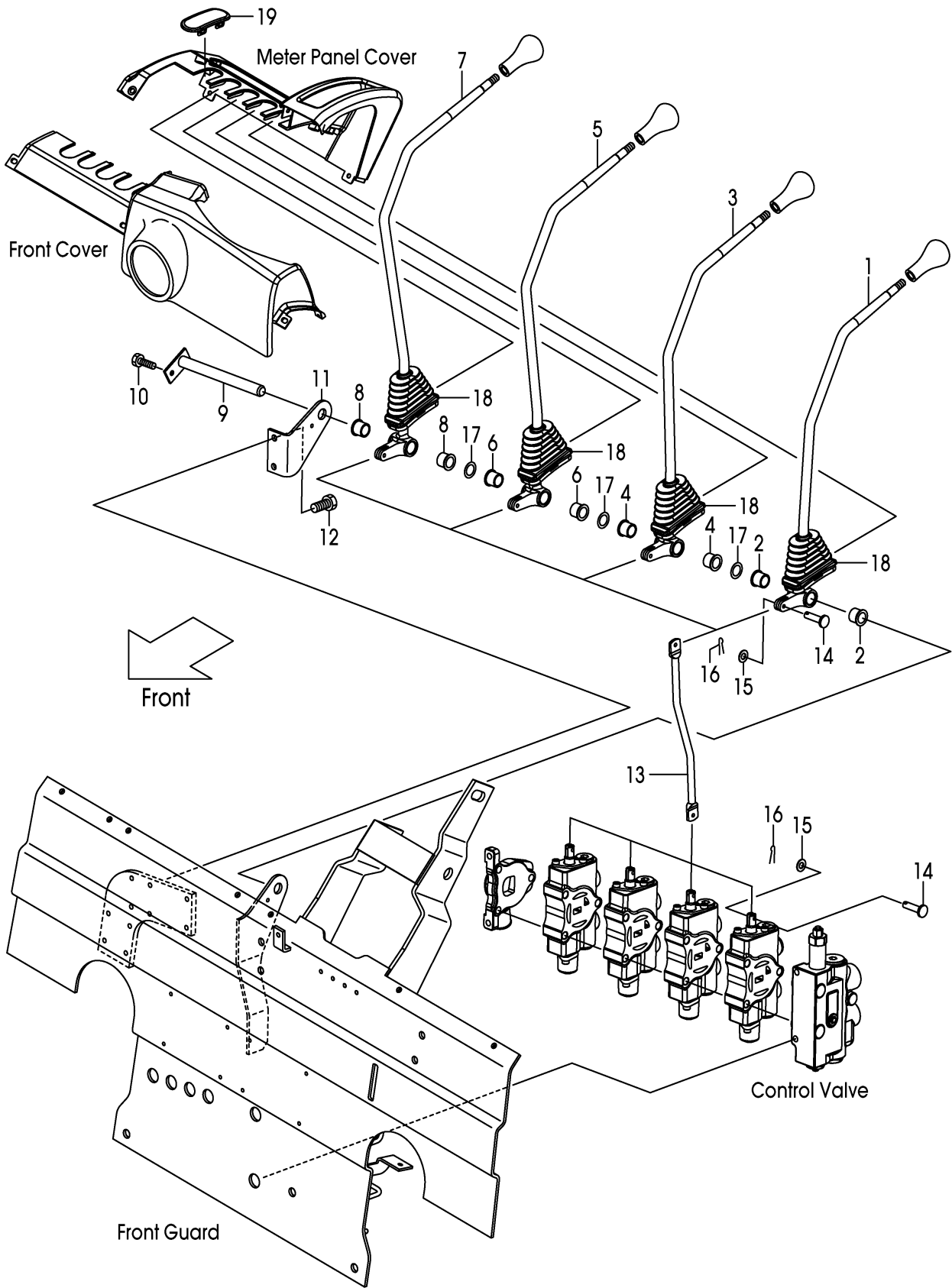
FIG.110 VALVE CONTROL [4SV] (F7G273C0)
