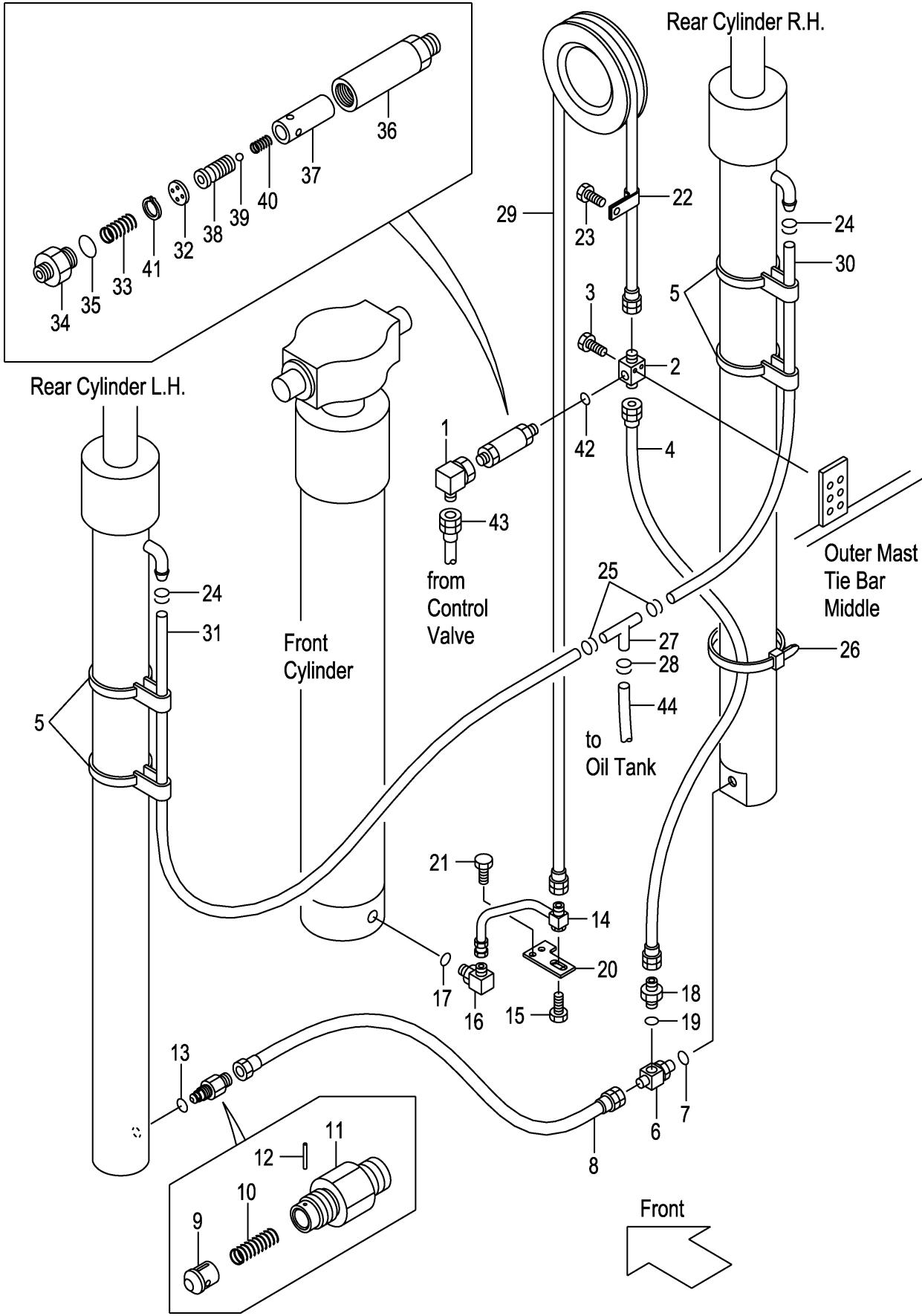
FIG.220 MAST PIPING [VFHMCN5] (M7G20830)
