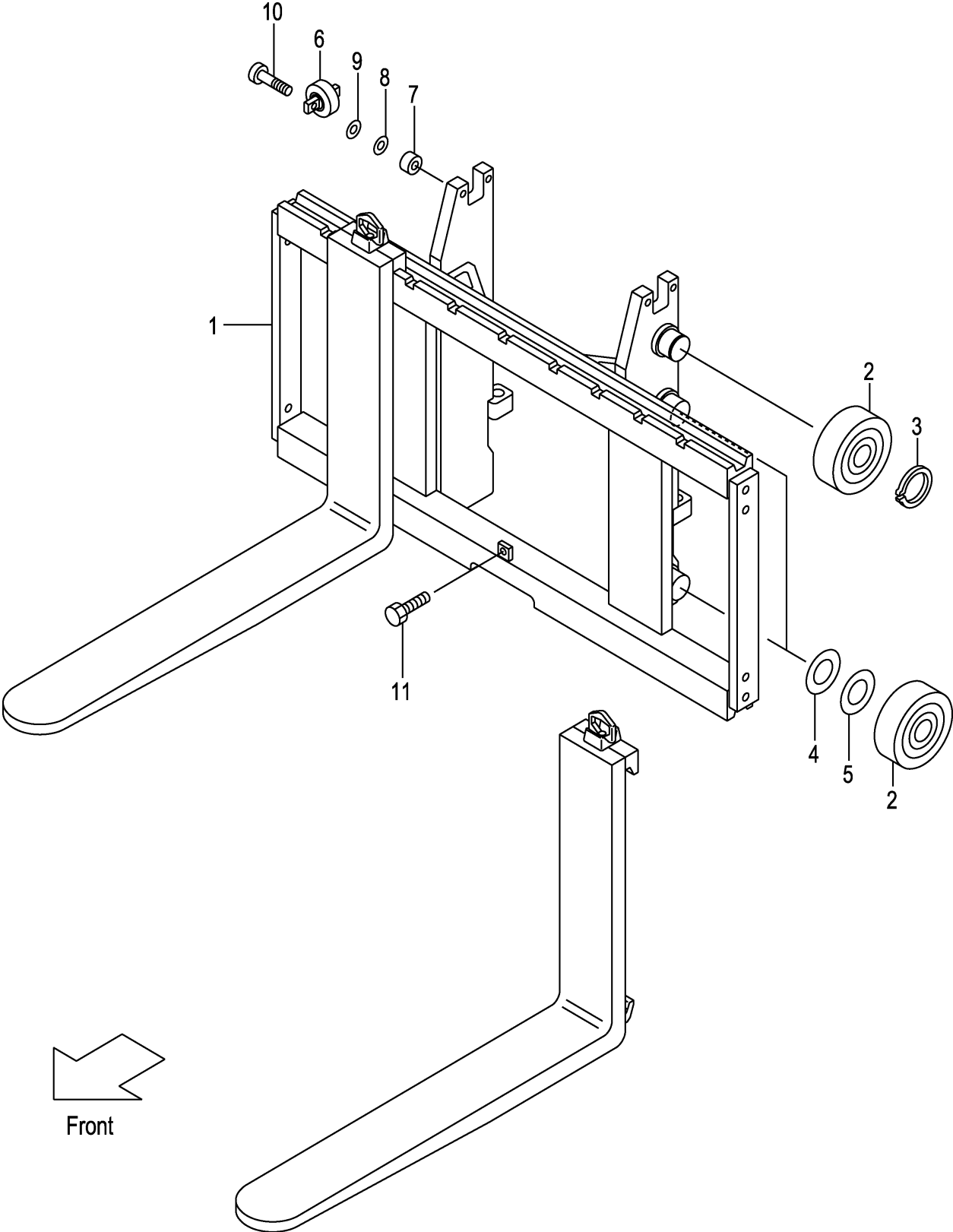
FIG.222 LIFT BRACKET [VMCN9] (M7G28230)
