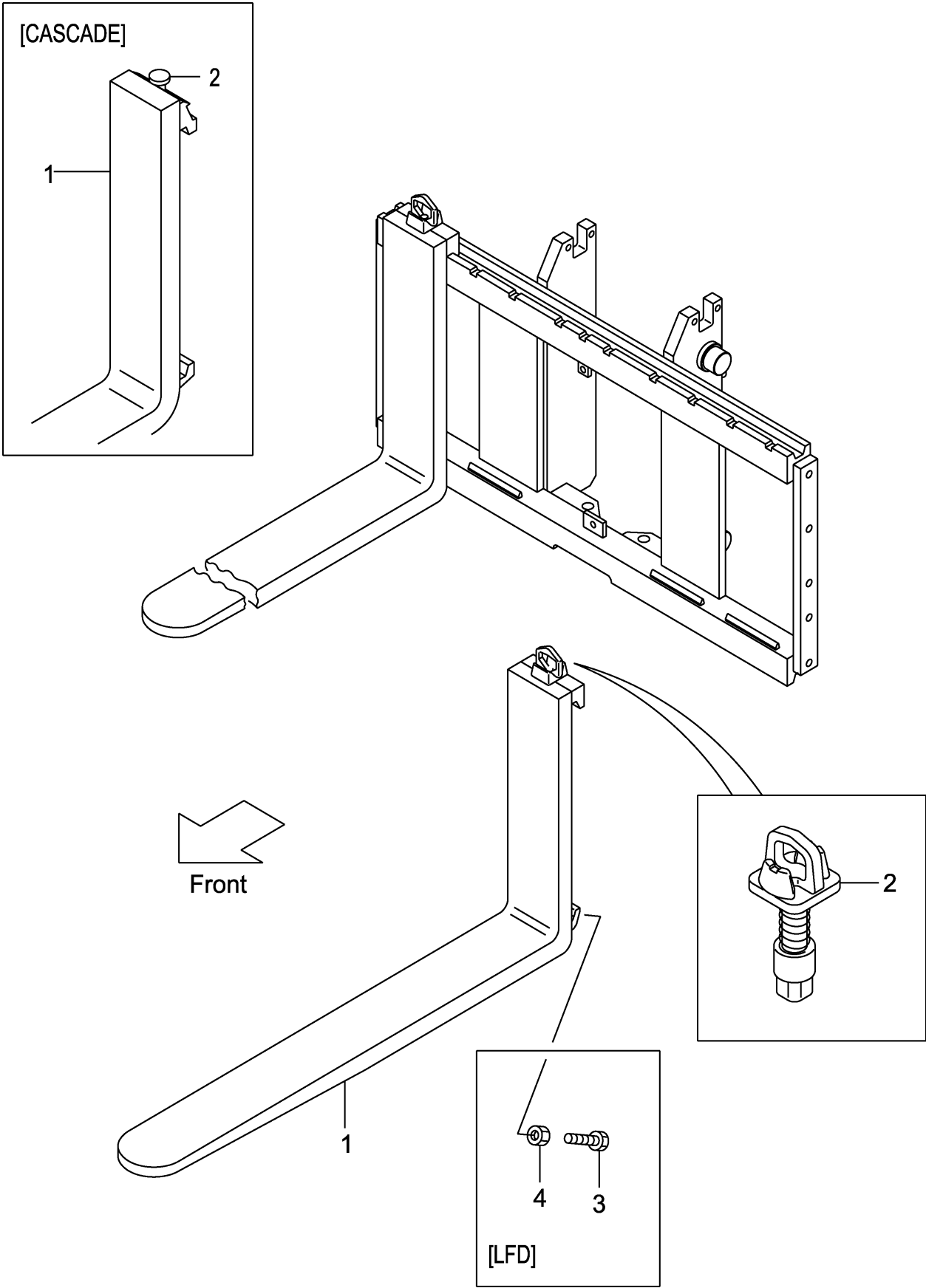
FIG.234 FORK [VFHMCN9] (M7G28180)
