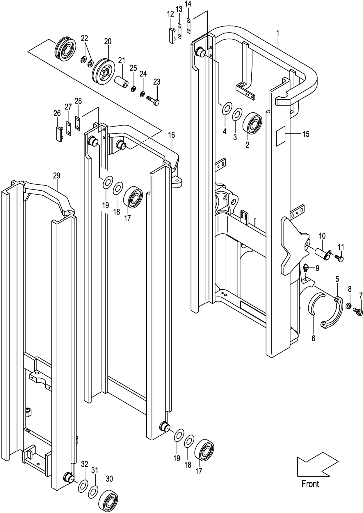
FIG.217 MAST [VFHMCN5] (M7G20710)
