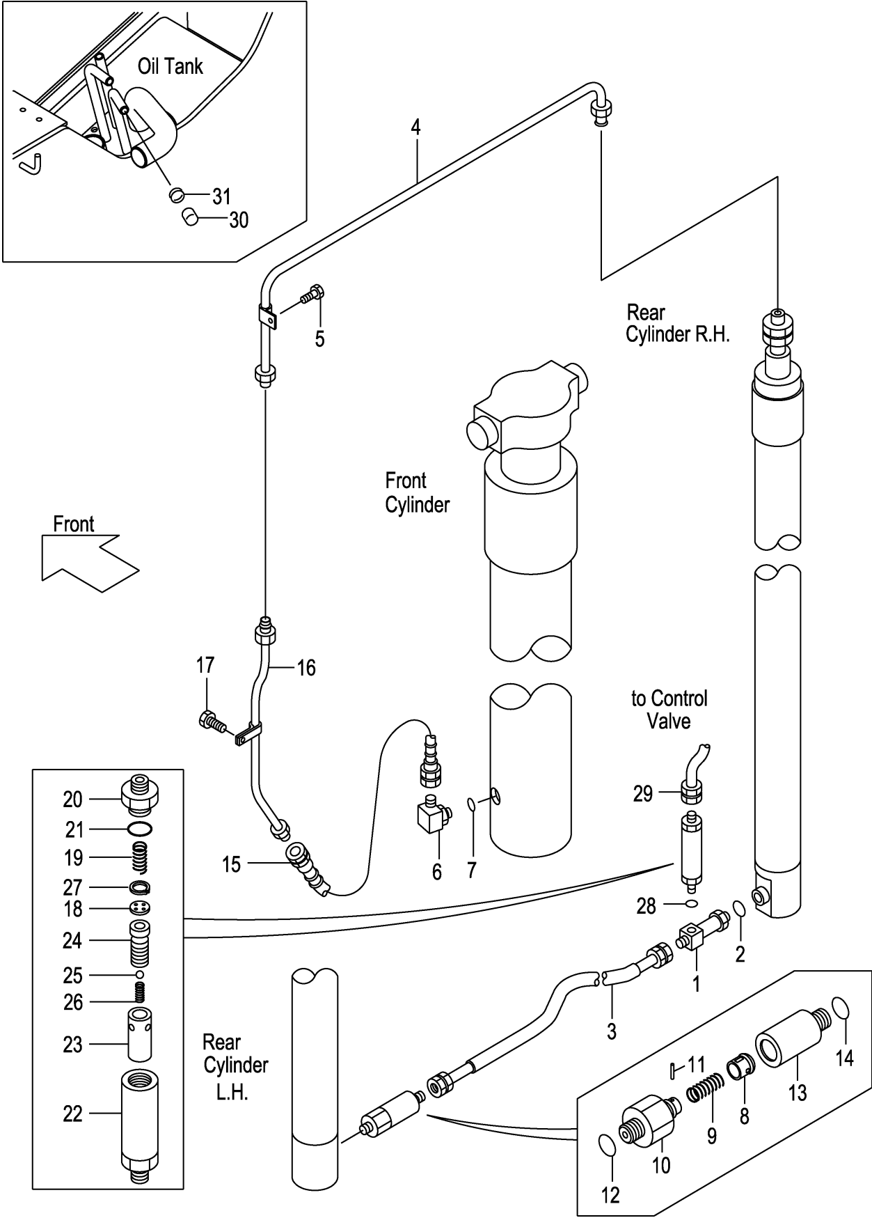
FIG.213 MAST PIPING [VFMCN5] (M7G20530)
