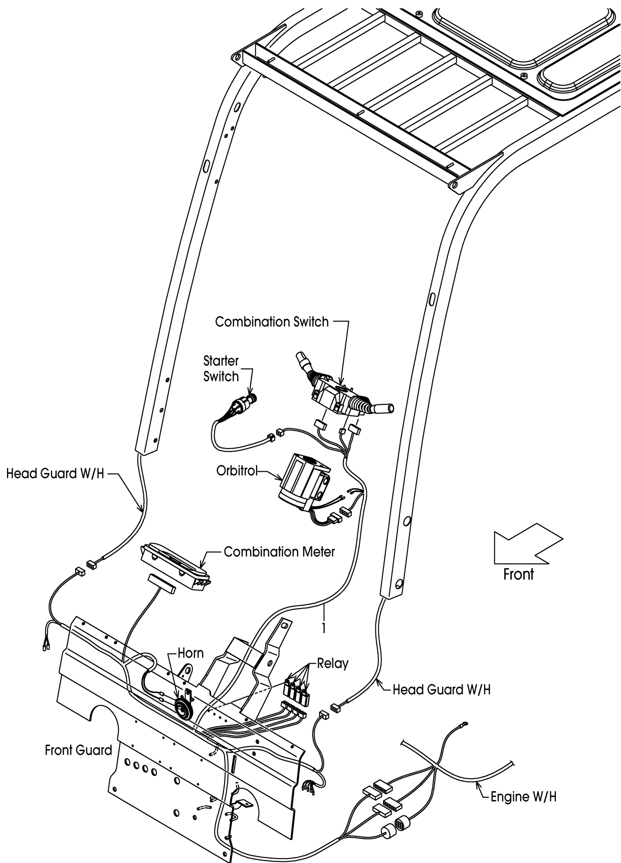
FIG.29 FRONT GUARD WIRE HARNESS (F7G22420)
