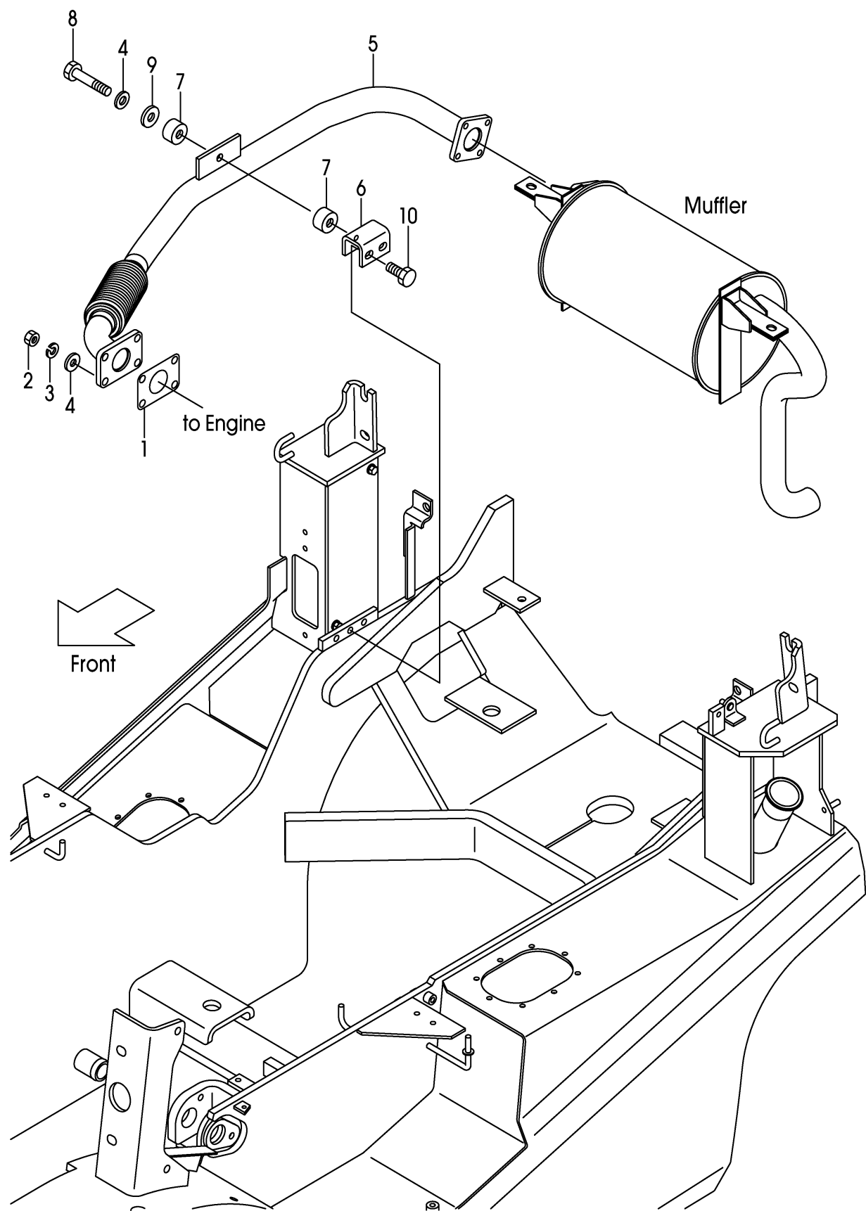
FIG.26 FRONT TUBE & JOINT (DIESEL) (F7G22350)
