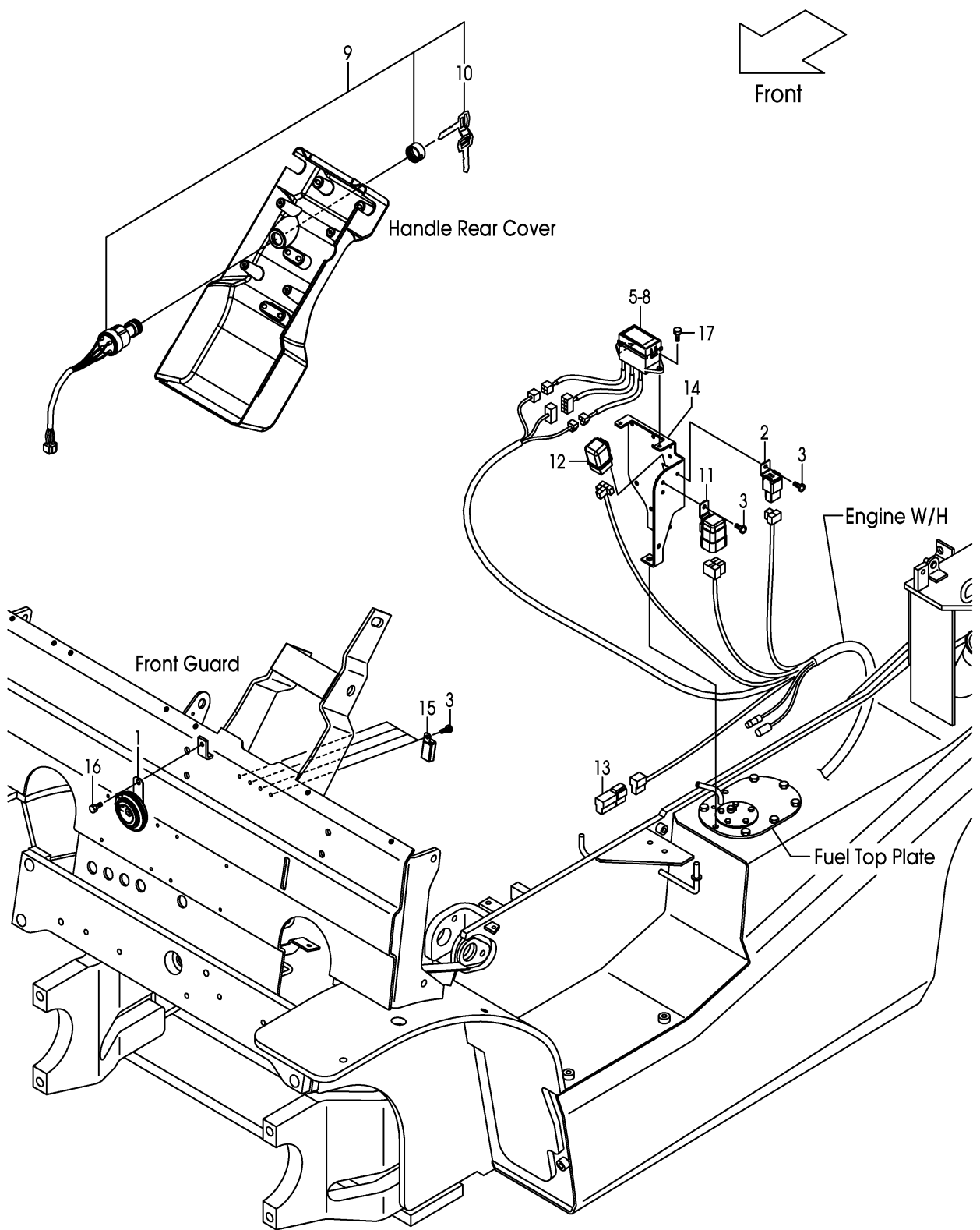
FIG.34 ELECTRIC PARTS (GASOLINE) (F7G22440)
