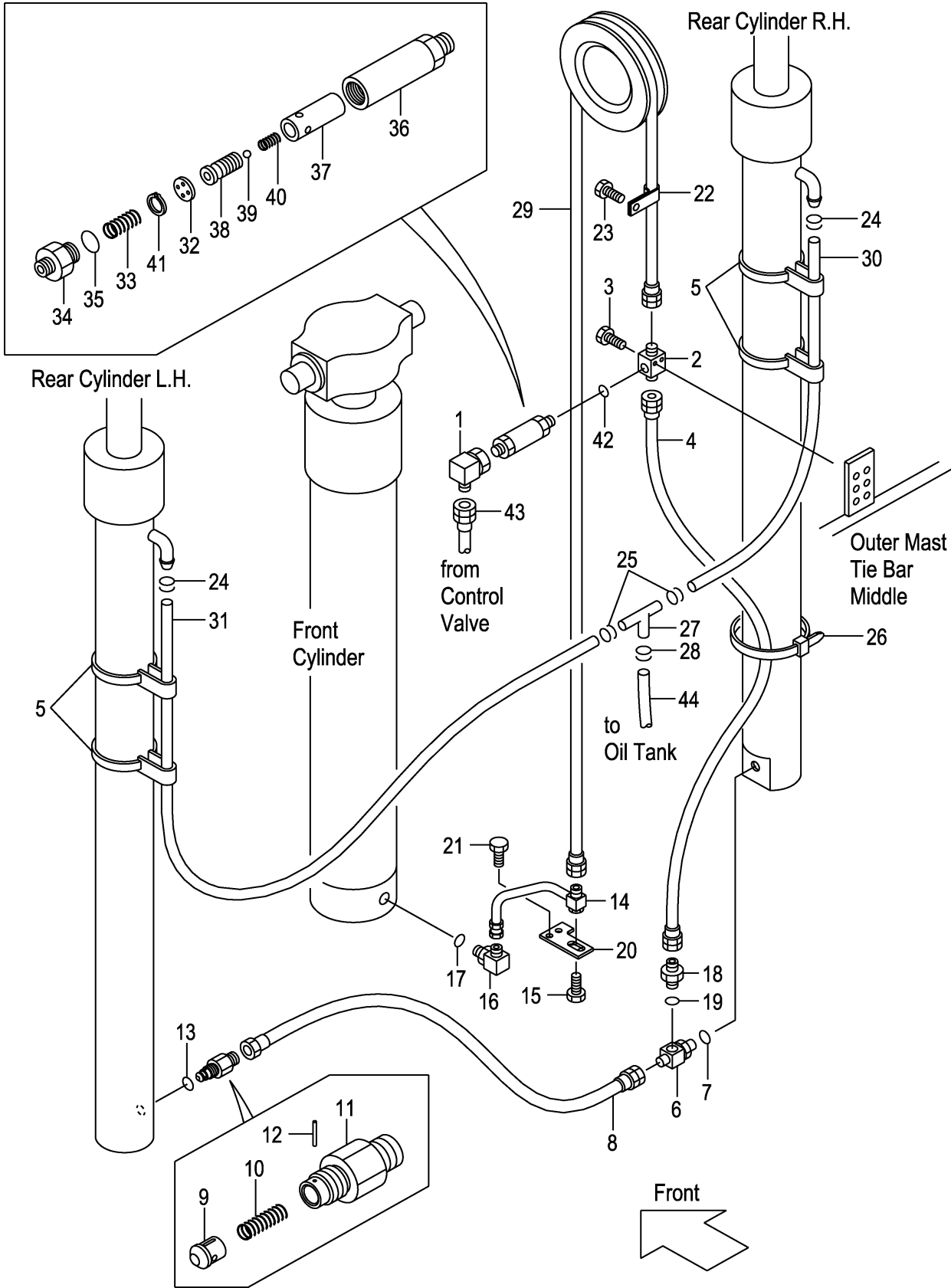
FIG.240 MAST PIPING [VFHMCN9] (M7G20890)
