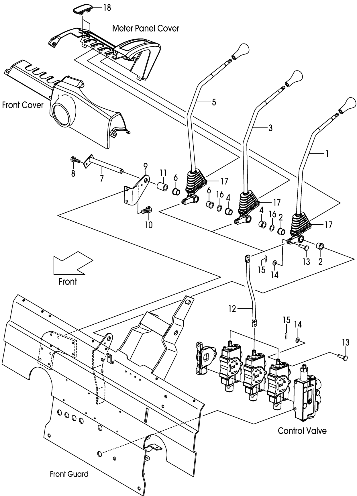
FIG.109 VALVE CONTROL [3SV] (F7G273B0)
