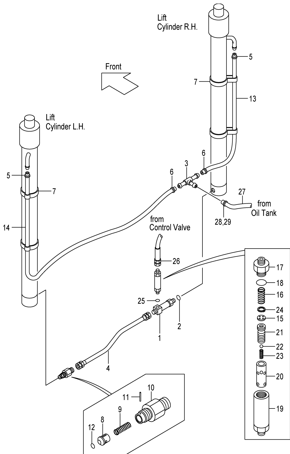
FIG.206 MAST PIPING [VMCN5] (M7G28420)
