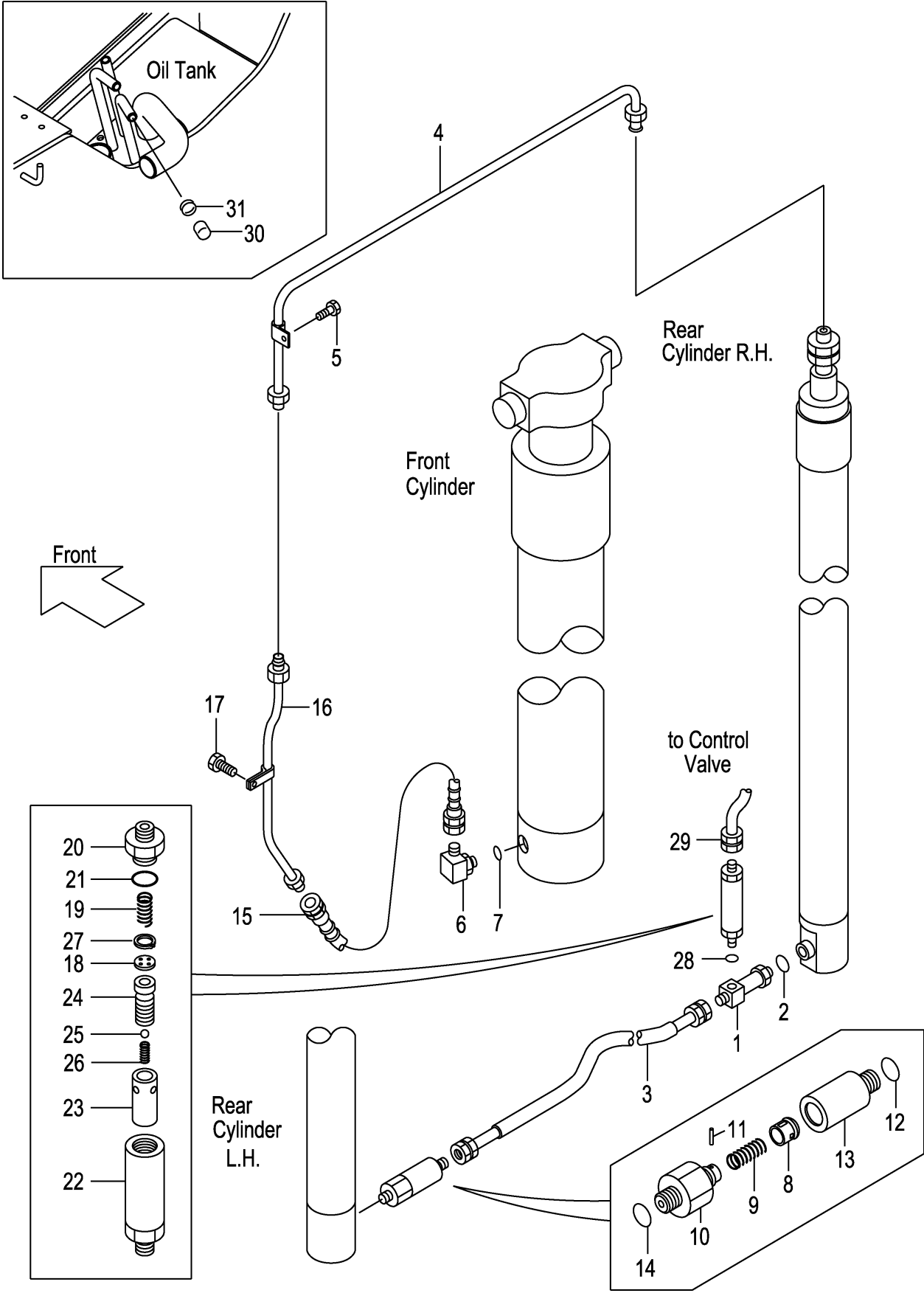
FIG.233 MAST PIPING [VFMCN9] (M7G20560)
