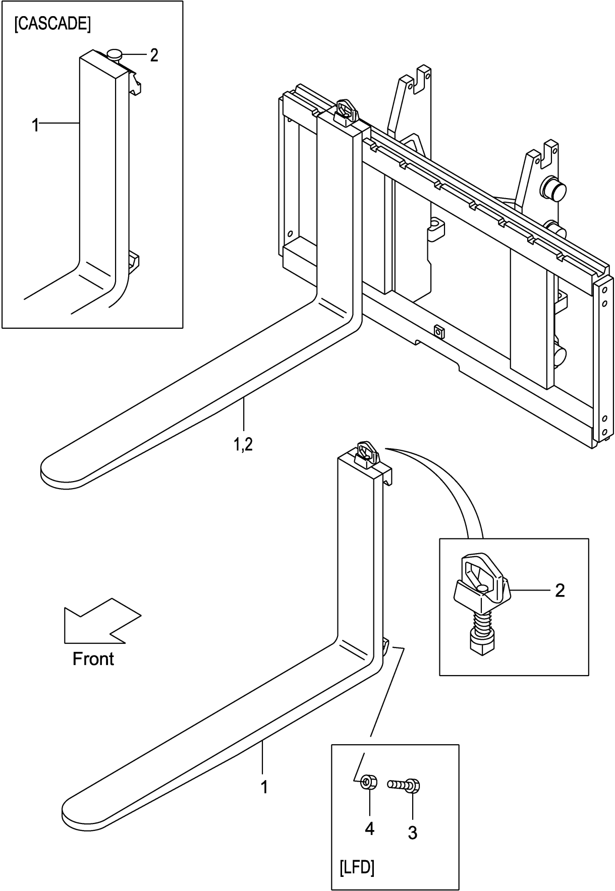
FIG.221 FORK [VMCN9] (M7G28120)
