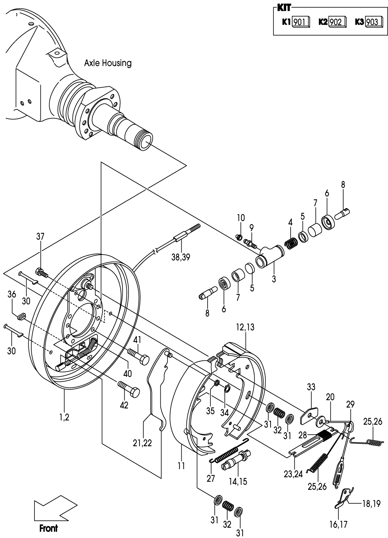
FIG.53 WHEEL BRAKE (F7G23720)
