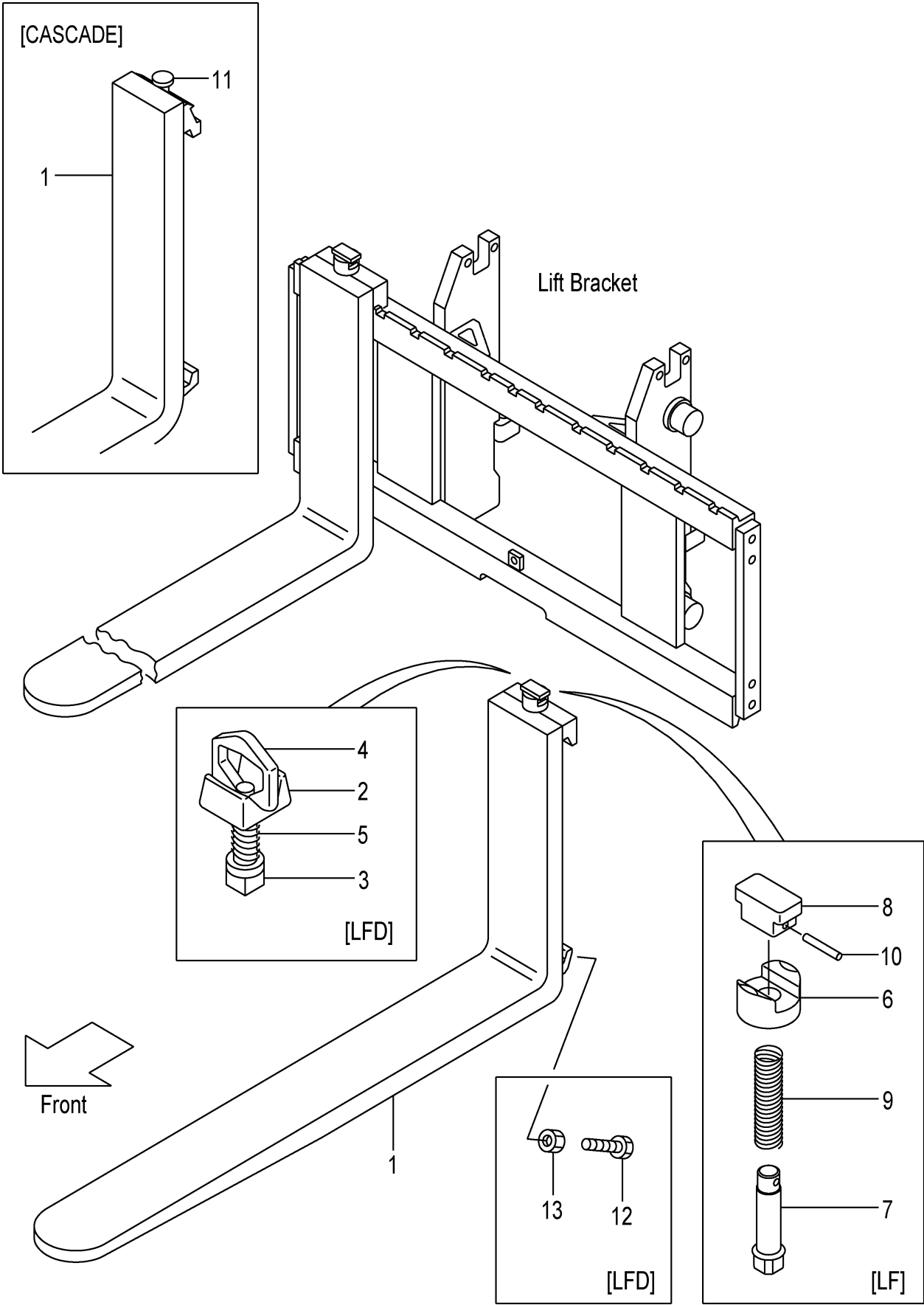
FIG.201 FORK [VMCN5] (M7G28110)
