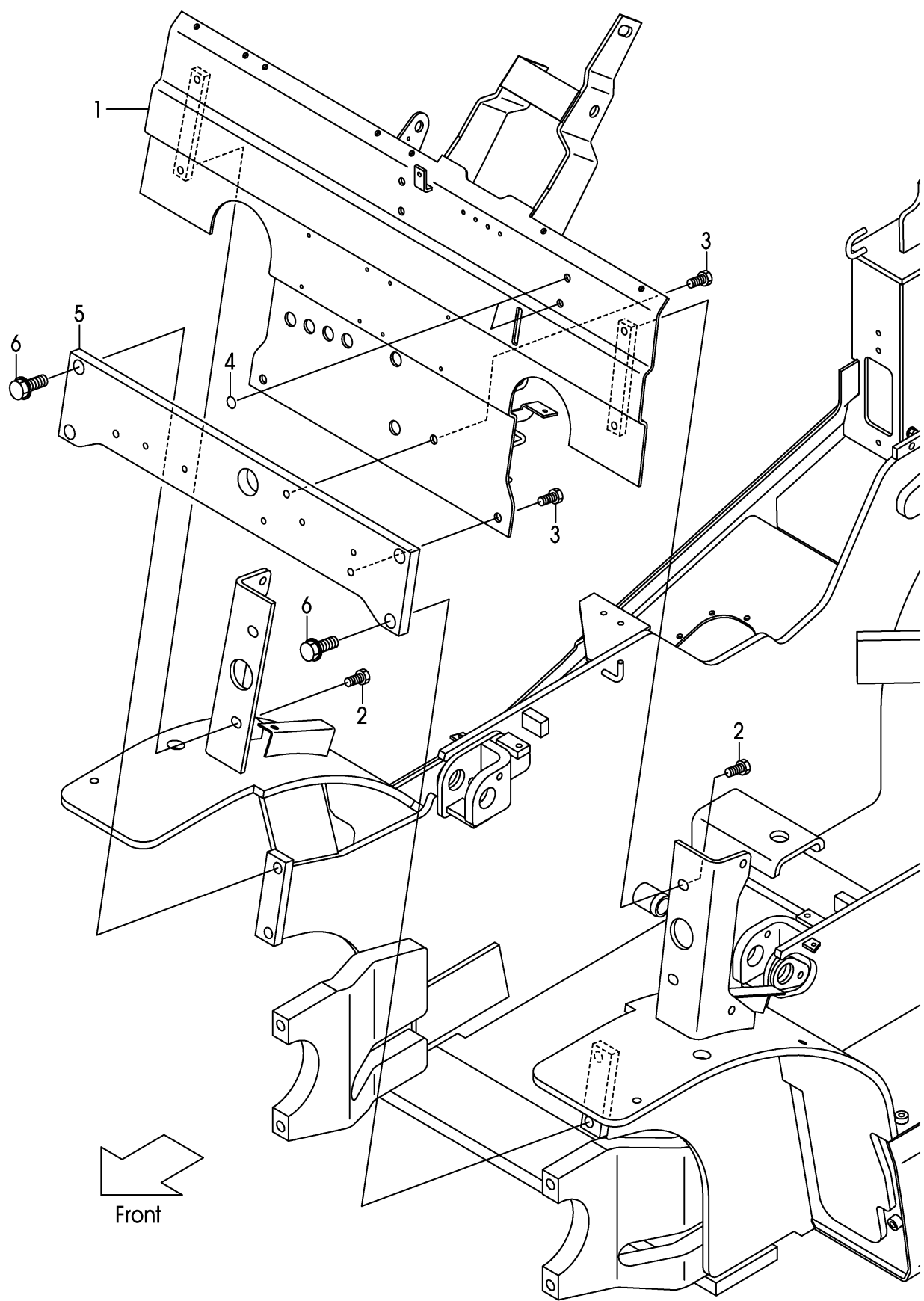
FIG.91 FRONT GUARD (F7G26410)
