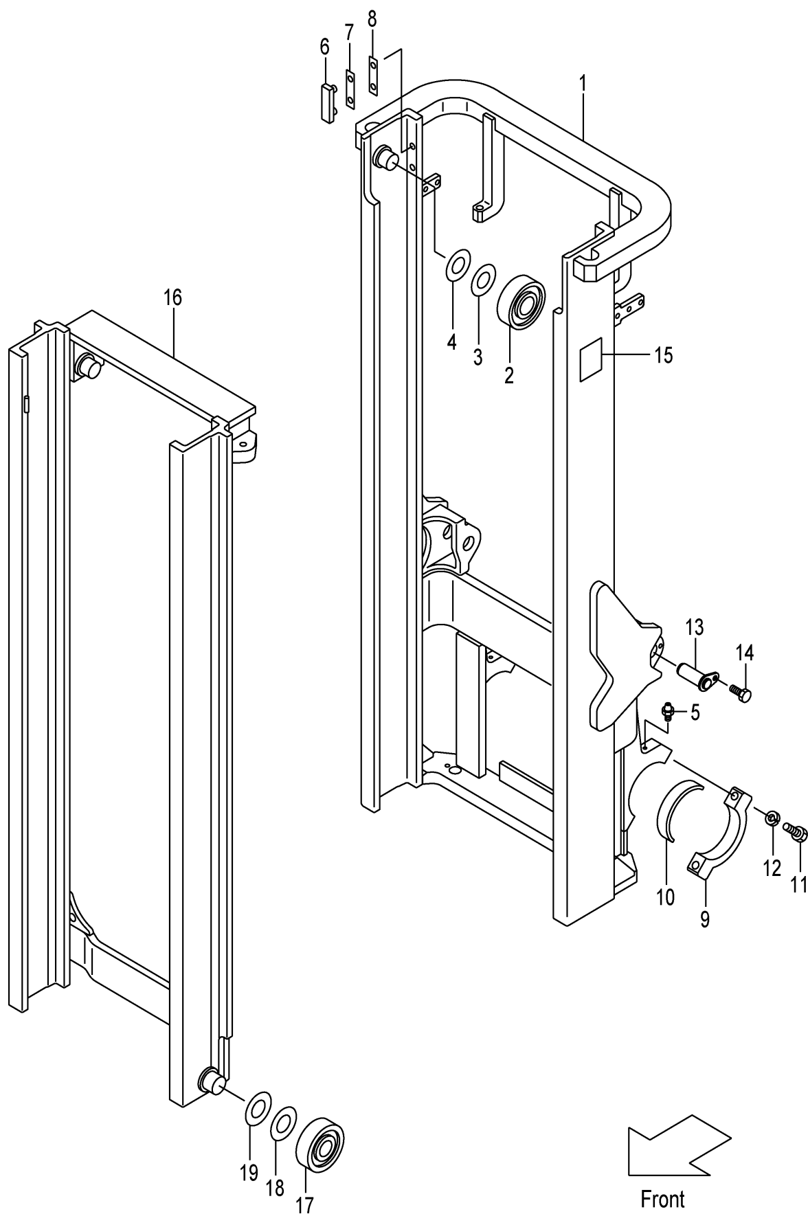
FIG.204 MAST [VMCN5] (M7G28310)
